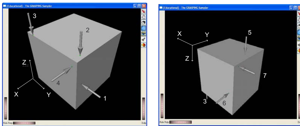
Fig. 7. Cube: Two views of the resulting fixturing (best trial).
