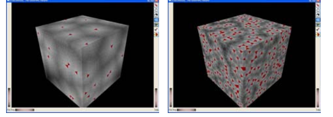
Fig. 3. Random sampling of the surface of a cube: 150 (left) and 500 samples (right).
