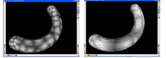
Fig. 4. Deterministic sampling (left) and random sampling (right) of the surface of a sausage using 150 samples.
