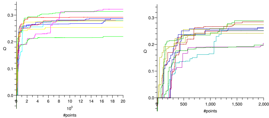
Fig. 6. Cube. Q for ten trials: evolution after visiting all the boundary triangles (left); zoom of the first 10% of visited triangles (right).
