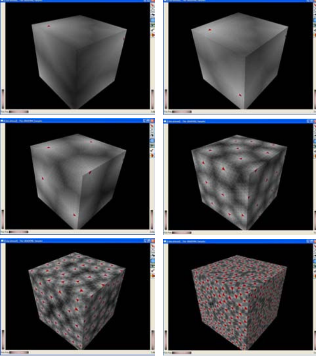
Fig. 2. Deterministic sampling of the surface of a cube (using 4, 5, 10, 50, 150 and 500 samples from left-top to bottom-right).
