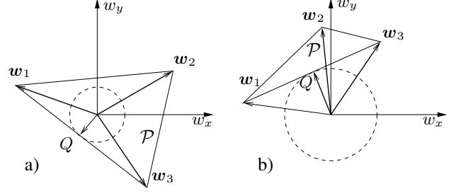
Fig. 5. Qualitative bidimensional example of \mathcal{P} and the grasp quality Q using three fingers: a) a FC-grasp ( O \in \mathcal{P} then Q > 0 ); b) a non FC-grasp ( O \notin \mathcal{P} then Q < 0 ).
